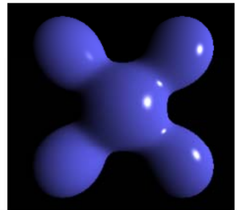
Phong Reflection
